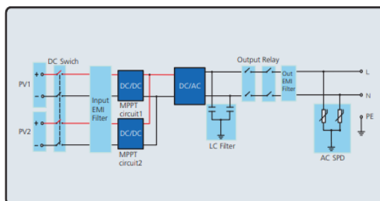
Growatt 2.5-3MTL-S topologia
